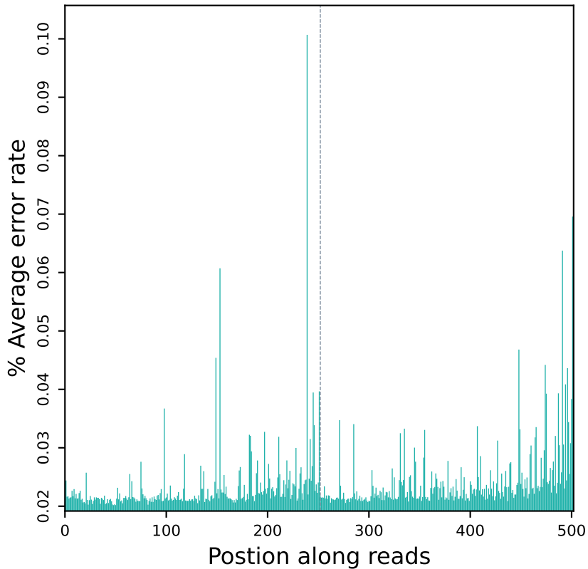
Error rate distribution along reads (R10918)
